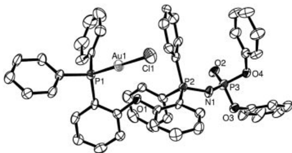
Figure 1. Molecular structure of [AuCl{κ 1 -P-Ph 2 PC 6 H 4 OC 6 H 4 PPh 2 =NP(O)(OPh) 2 }] ( 10 ). All hydrogen atoms have been omitted for clarity. Thermal ellipsoids are drawn at the 50% probability level.
