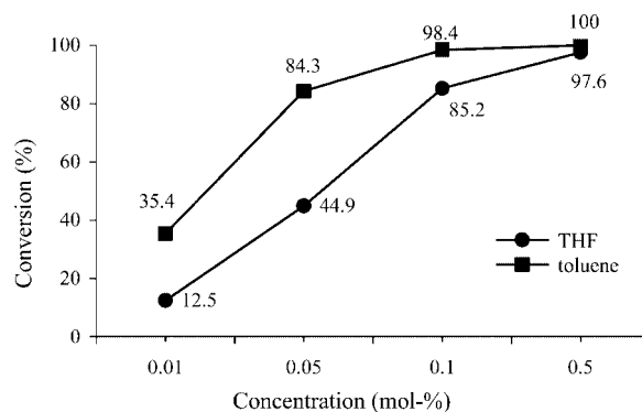
Figure 2. Influence of catalyst concentration on the coupling of 4-bromobenzaldehyde (1.0 mmol) and phenylboronic acid (1.5 mmol). Conditions: K 3 PO 4 (2.0 mmol), toluene/thf (10 mL), t = 15 min, T = 70 °C.
