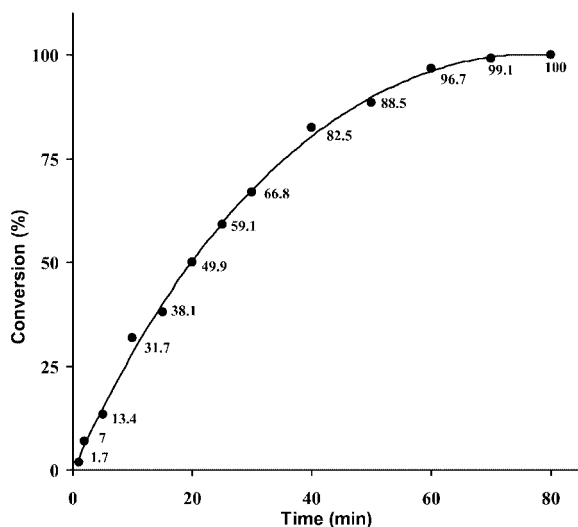
Figure 3. Hydrogenation of styrene. Conditions: styrene (1.0 mmol), \text{Et}_3\text{N} (0.1 mmol), 11 (0.0005 mol-%), thf (20 mL); \text{H}_2 pressure: 4 atm; room temperature; stirring speed: 400 rpm.
